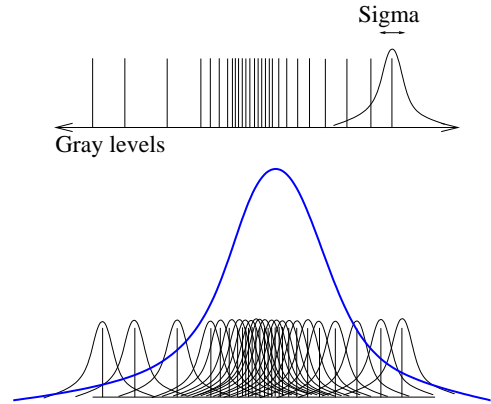
Figure 8.47: In Parzen windowing, a continuous density function is constructed by superimposing kernel functions (Gaussian function in this case) centered on the intensity samples obtained from the image.
