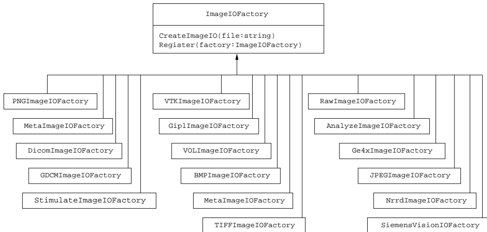
Figure 7.3: Class diagram of the ImageIO factories.
