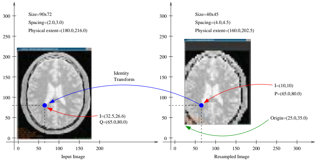
Figure 6.50: Effect of non-unit spacing on the input and output images.
