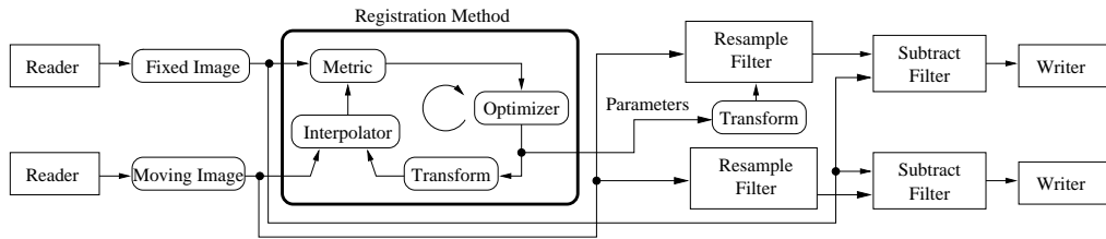
Figure 8.5: Pipeline structure of the registration example.
