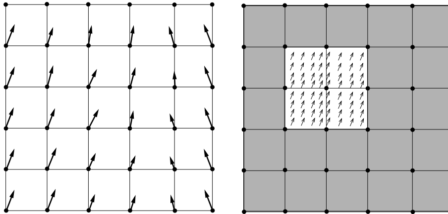
Figure 8.45: The left side illustrates the B-spline grid and the deformations that are known on those nodes. The right side illustrates the region where interpolation is possible when the B-spline is of cubic order. The small arrows represent deformation values that were interpolated from the grid deformations shown on the left side of the diagram.
