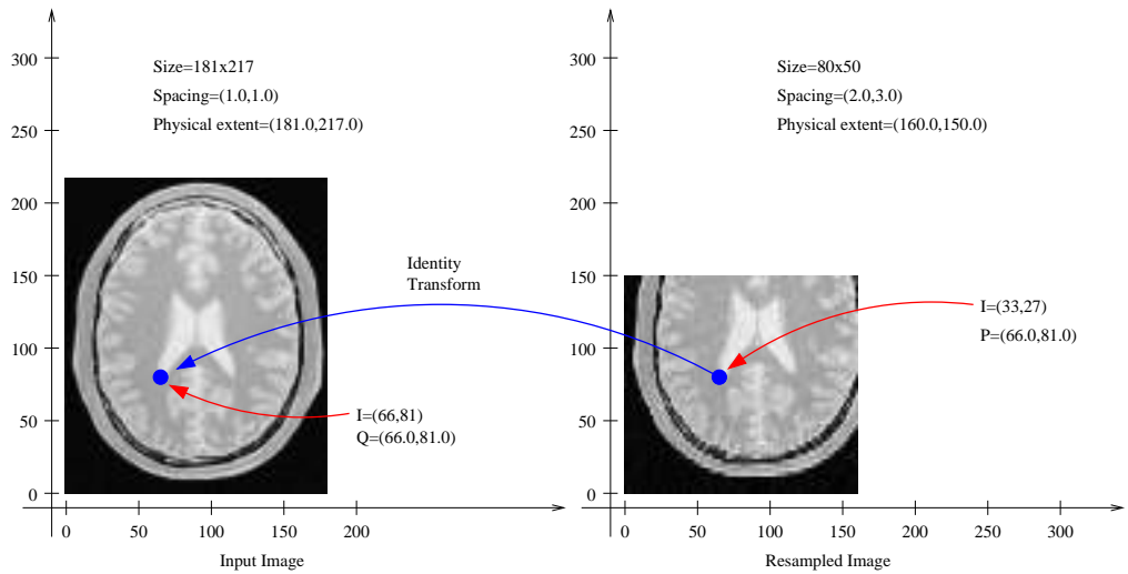
Figure 6.48: Effect of selecting the spacing on the output image.
