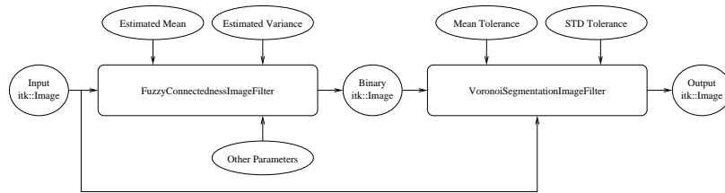
Figure 9.41: Integration of the fuzzy connectedness and Voronoi segmentation filters.
