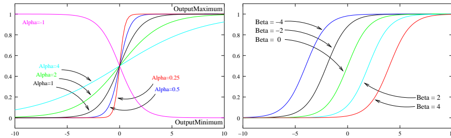
Figure 6.6: Effects of the various parameters in the SigmoidImageFilter . The alpha parameter defines the width of the intensity window. The beta parameter defines the center of the intensity window.
