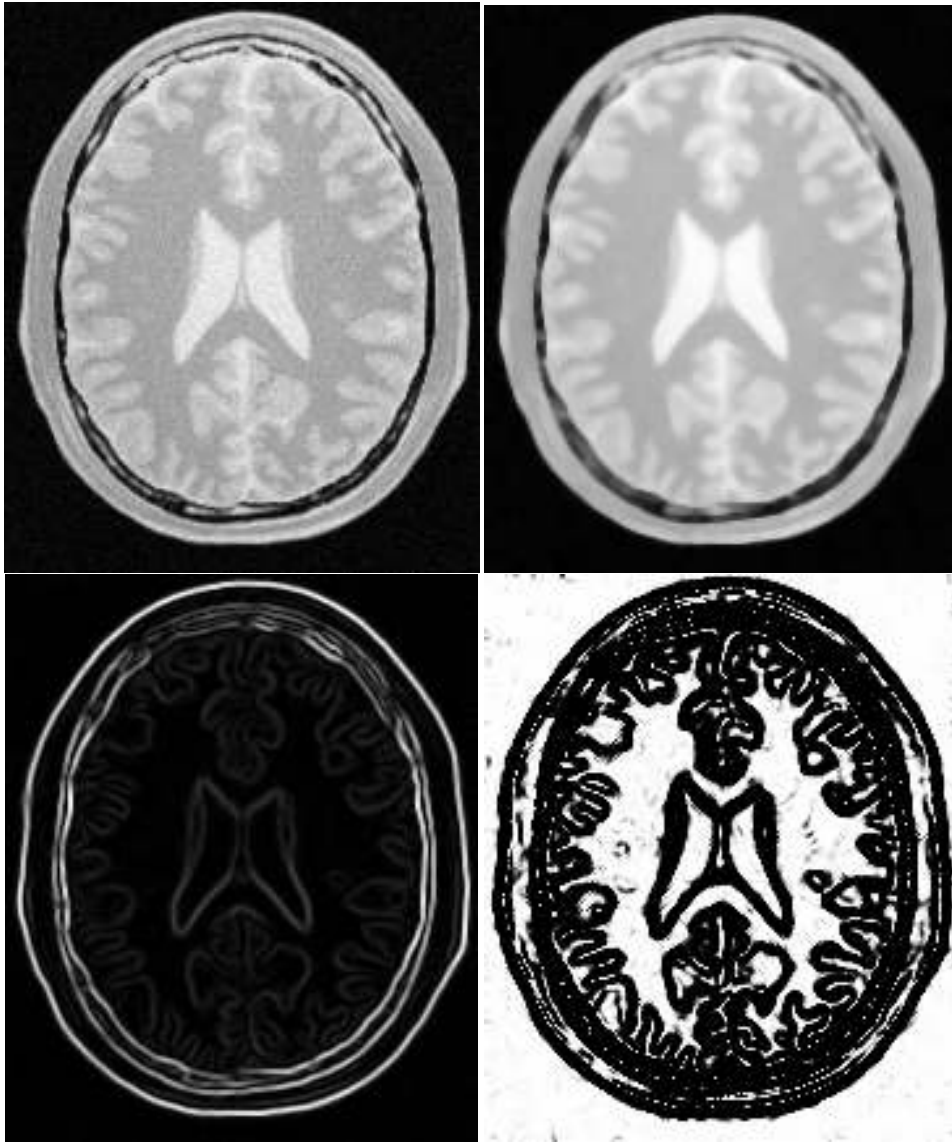
Figure 9.16: Images generated by the segmentation process based on the FastMarchingImageFilter . From left to right and top to bottom: input image to be segmented, image smoothed with an edge-preserving smoothing filter, gradient magnitude of the smoothed image, sigmoid of the gradient magnitude. This last image, the sigmoid, is used to compute the speed term for the front propagation
