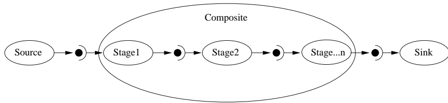
Figure 13.4: A Composite filter encapsulates a number of other filters.
