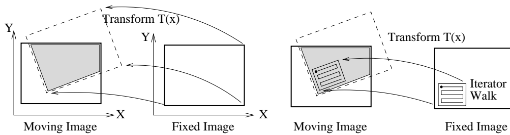
Figure 8.43: The moving image is mapped into the fixed image space under some spatial transformation. An iterator walks through the fixed image and its coordinates are mapped onto the moving image.
