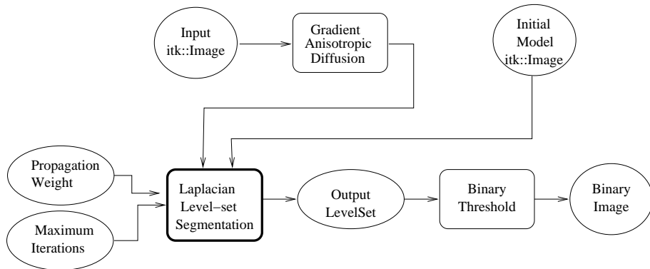
Figure 9.29: An image processing pipeline using LaplacianSegmentationLevelSetImageFilter for segmentation.
