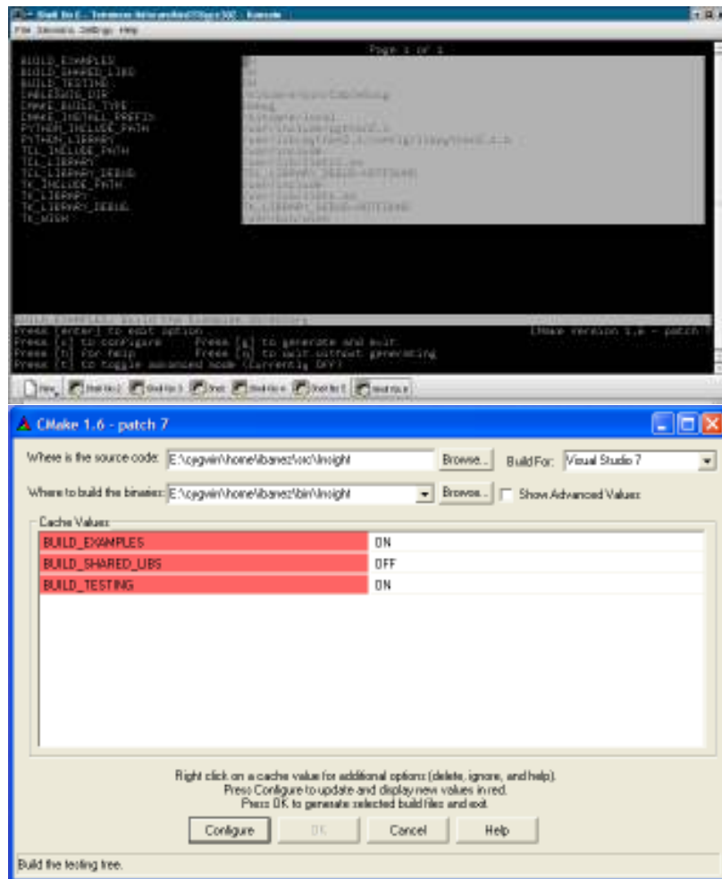
Figure 2.1: CMake interface. Top) ccmake, the UNIX version based on curses. Bottom) CMakeSetup, the MS-Windows version based on MFC.
