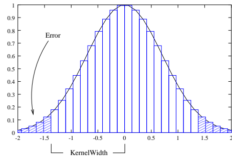
Figure 6.21: Discretized Gaussian.
